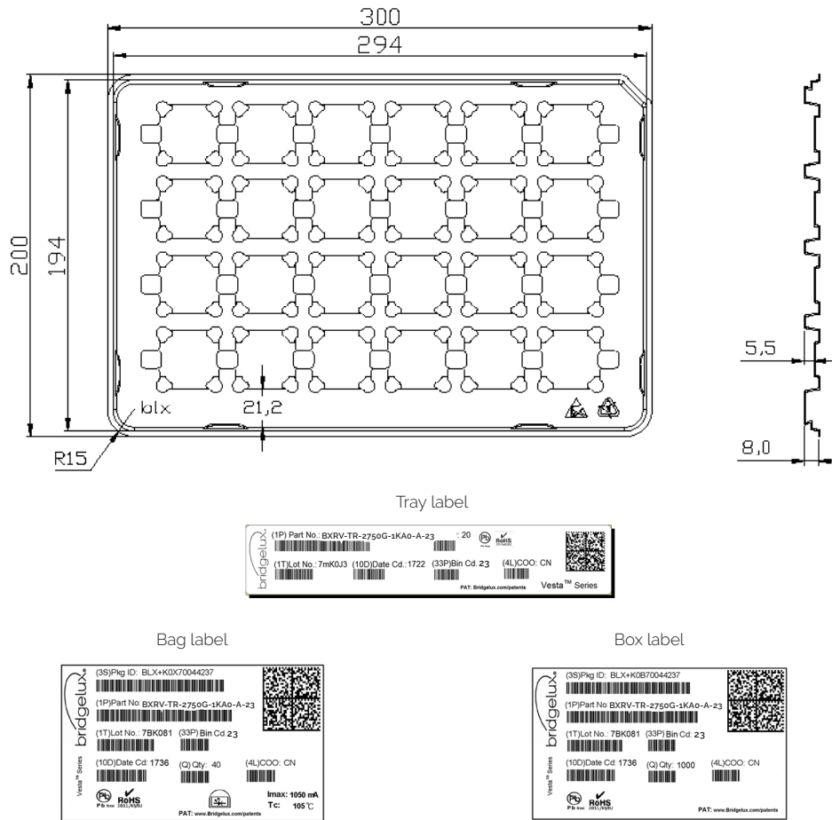
Figure 17: Vesta Series Tunable White 29mm Packaging and Labeling
