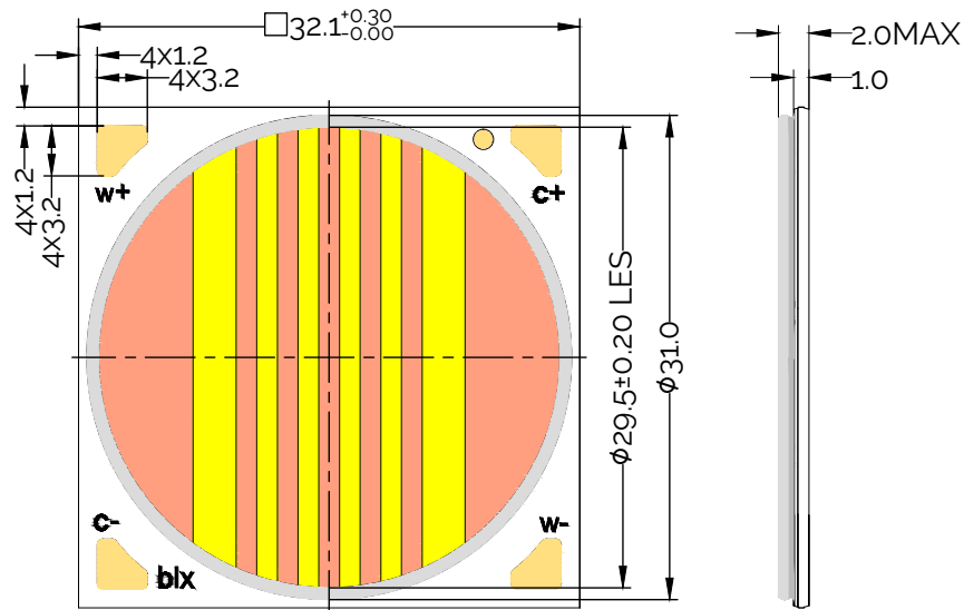
Figure 14: Drawing for Vesta Series Tunable White Gen 2 29mm Array
